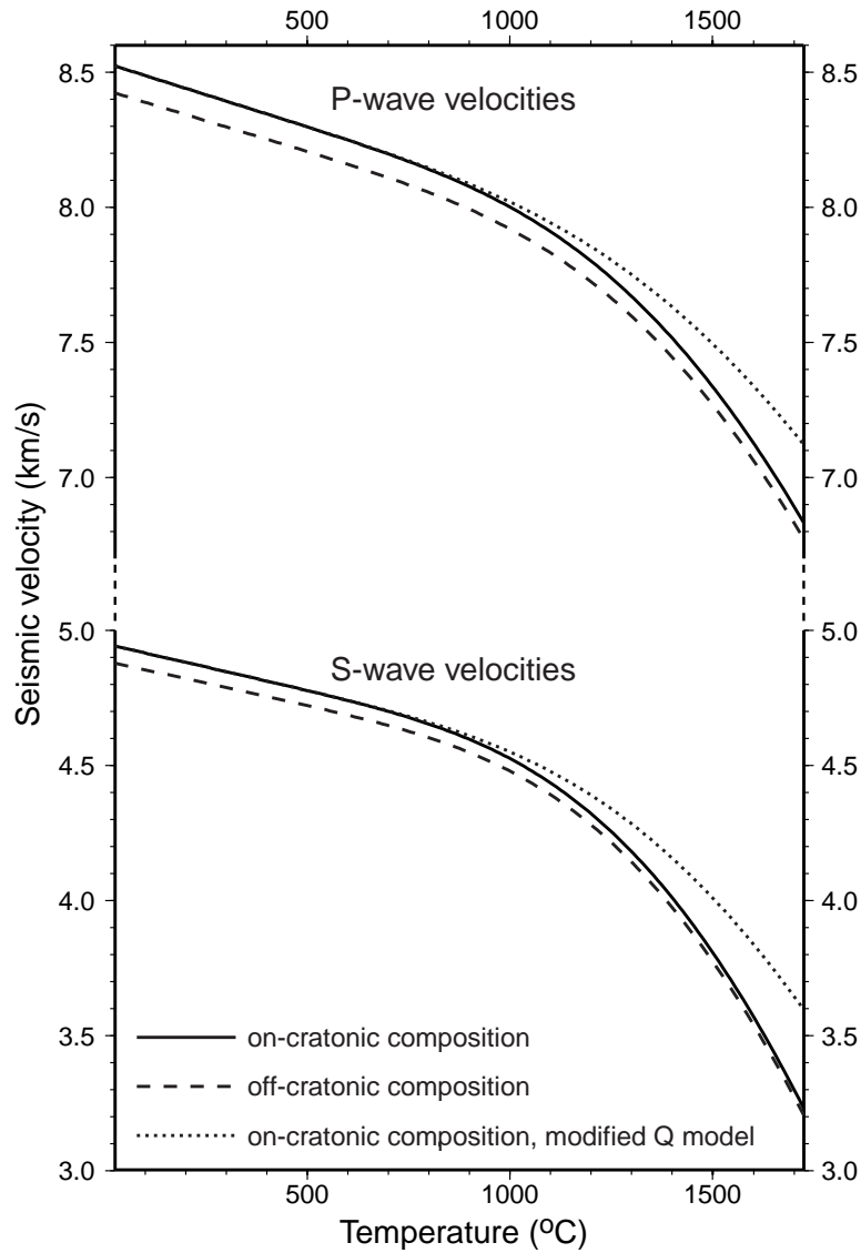
Figure 3. P - and S -wave velocities calculated at 60 km depth using equations (A1)-(A13). Solid lines show the results for on-cratonic composition with the “normal” anelastic correction ( A = 0.049 ). Dashed lines show the results for the off-cratonic composition with the “normal” anelastic correction. Dotted lines are the results for the on-cratonic composition with a “reduced” anelastic correction ( A = 0.074 ).
