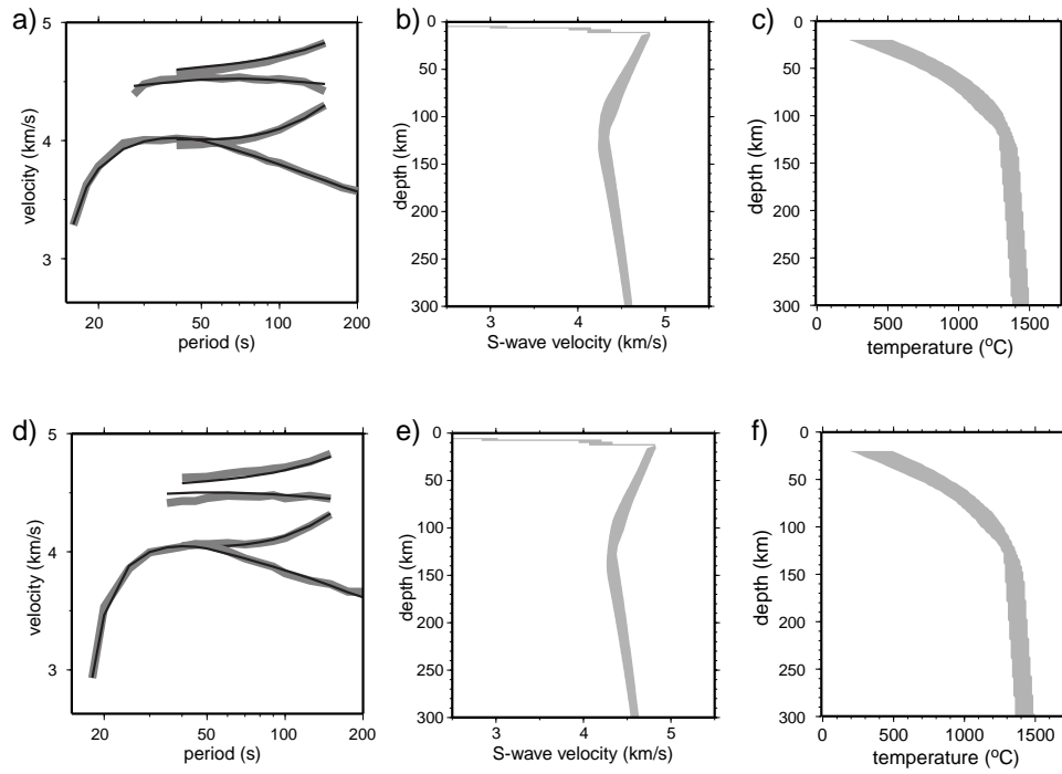
Figure 14. Results of the surface-wave inversion with the thermal parameterization at two locations in the Pacific Ocean (44S, 134W) and (32N, 160W), similar to Figure 11.
