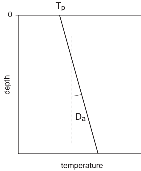
Figure A2. Schematic geotherm in the convective mantle, see equation (B1), where T_p is potential temperature, D_a is the adiabatic gradient, and depth and temperature range over values appropriate to the convective part of the model (see Figure 10).
