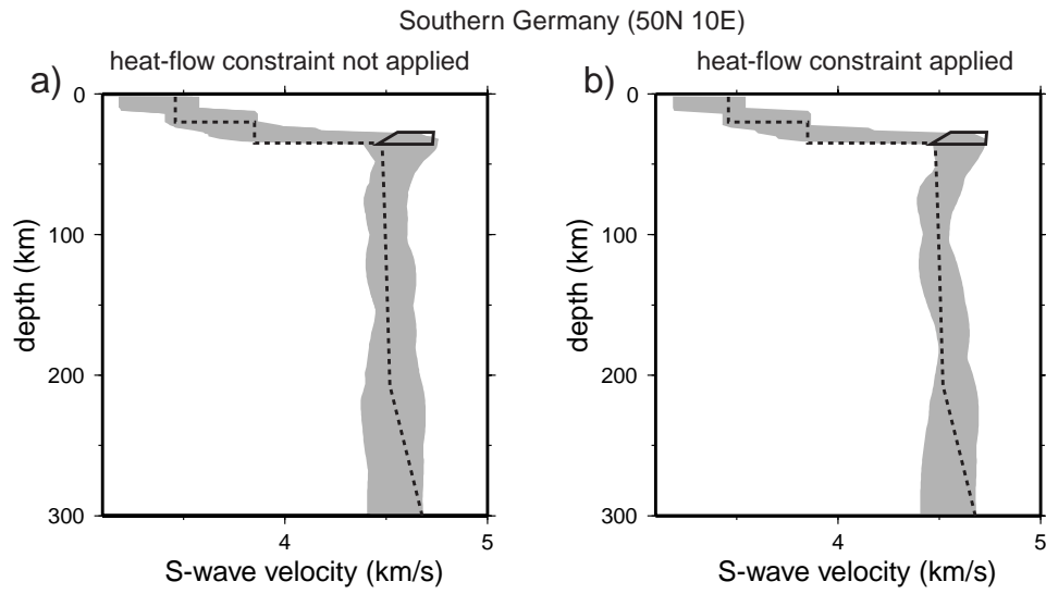
Figure 8. Similar to Figure 6, but for a region that has undergone recent tectonic deformation, a location in Southern Germany (50N, 10E).
