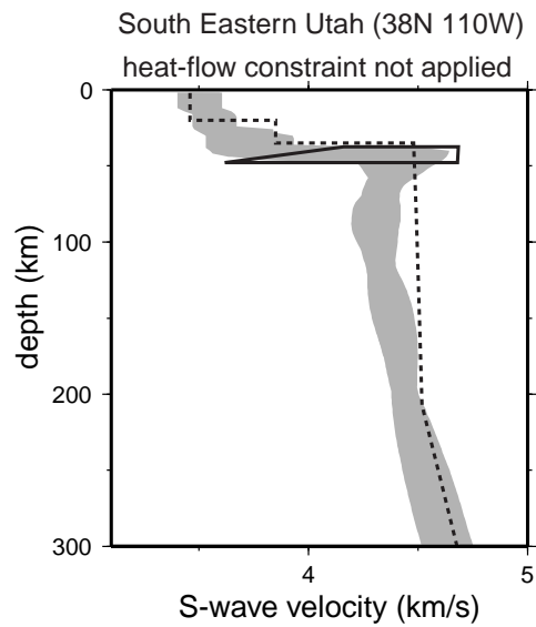
Figure 9. Similar to Figure 6, but for a second region that has undergone recent tectonic deformation, a location in Southeastern Utah (38N, 110W). The heat flow constraint does not change the ensemble of acceptable models from those that result from seismic data alone, so only a single panel is shown.
