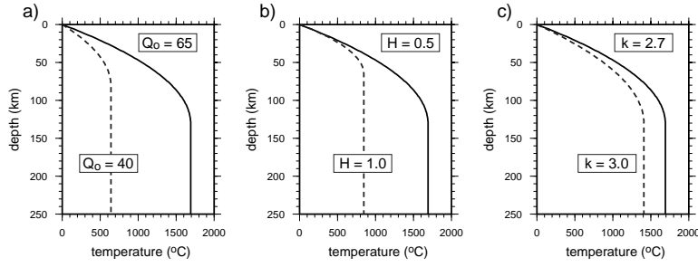
Figure A3. Solutions of the 1D thermal steady-state equation (B5) with boundary conditions (B4) and (B6). (a) Effect of surface heat flow. Solid and dashed lines show solutions obtained with Q_0 = 65 \text{mW}/\text{m}^2 and Q_0 = 40 \text{mW}/\text{m}^2 , respectively. In both cases, H = 0.5 \mu\text{W}/\text{m}^3 and k = 2.7 \text{Wm}^{-1}\text{K}^{-1} . (b) Effect of internal heat production. Solid and dashed lines show solutions obtained with H = 0.5 \mu\text{W}/\text{m}^3 and H = 1.0 \mu\text{W}/\text{m}^3 , respectively. In both cases, Q_0 = 65 \text{mW}/\text{m}^2 and k = 2.7 \text{Wm}^{-1}\text{K}^{-1} . (c) Effect of thermal conductivity. Solid and dashed lines show solutions obtained with k = 2.7 \text{Wm}^{-1}\text{K}^{-1} and k = 3.0 \text{Wm}^{-1}\text{K}^{-1} , respectively. In both cases, Q_0 = 65 \text{mW}/\text{m}^2 and H = 0.5 \mu\text{W}/\text{m}^3 .
