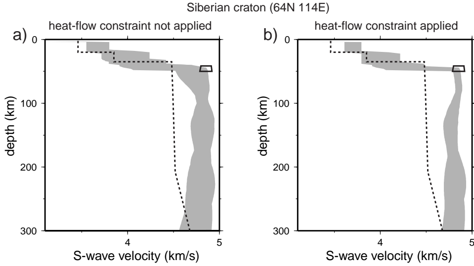
Figure 6. Results of the surface wave inversion at a location in the Siberian craton (64N, 114E). The shaded zones identify the ensemble of acceptable models for isotropic shear velocity ( v_s = (v_{sh} + v_{sv})/2 ). The dashed lines are the 1-D model ak135 (Kennett et al. 1995), for reference. Black polygons mark the area of allowed shear velocities at the top of the mantle estimated from the heat flow data. (a) Results without the heat-flow constraint. The black polygon is included for reference only. (b) Results with the heat flow constraint. All models pass through the black polygon.
