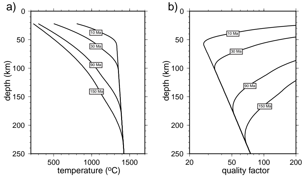
Figure 13. Thermal models of the sub-oceanic upper mantle with a potential temperature T_p = 1300^\circ\text{C} and four different cooling ages: 10 Ma, 30 Ma, 90 Ma, and 150 Ma. (a) Temperature as a function of depth. (b) Shear quality factor as a function of depth.
