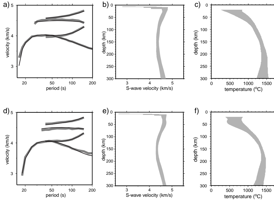
Figure 11. The seismic model and inferred temperature at two locations in the Pacific using the ad-hoc seismic parameterization of Shapiro & Ritzwoller (2002). (a-c) Results of the surface-wave inversion for a location in the Southern Pacific Ocean (44S, 134W). (a) Dispersion curves, similar to Figure 1a. (b) The shaded area defines the ensemble of acceptable models (isotropic part, v_s = (v_{sv} + v_{sh})/2 ). (c) The shaded area defines the allowed temperatures predicted from the ensemble of acceptable seismic models. (d-f) Similar to (a-c), but for a location in the Northern Pacific (32N, 160W).
