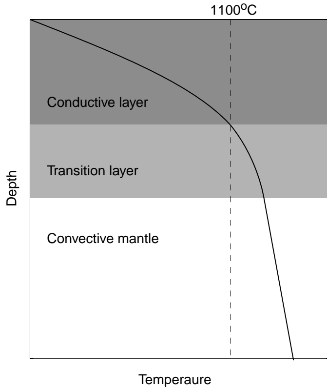
Figure 10. Model of the sub-oceanic upper mantle used to define the thermal parameterization. The solid line represents an allowed temperature profile.
