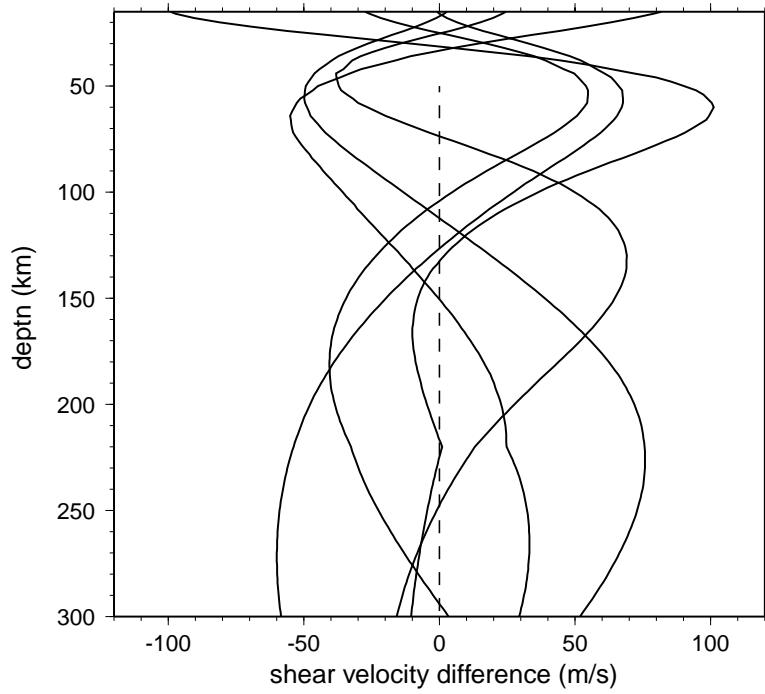
Figure 12. Differences in shear velocities between five randomly selected pairs of acceptable models at the northern Pacific location (32N, 160W). These profiles are in the effective null-space of the data.
